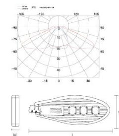
配光曲线 Light distribution curve
